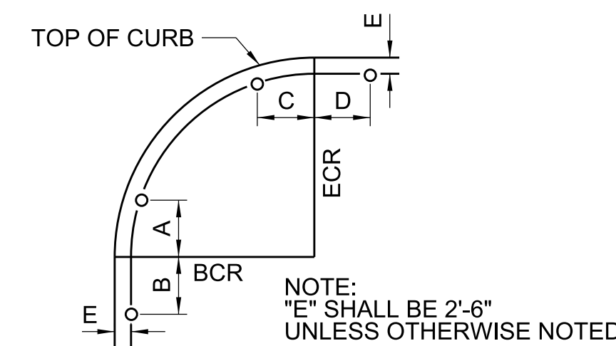
POLE LOCATION DETAIL NOT TO SCALE
